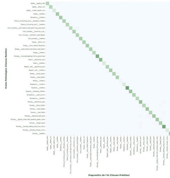
Figure 3: Global 38x38 Confusion Matrix on independent validation data — Strong diagonal concentration confirms model discriminative power
