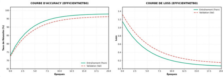
Figure 2: Multi-epoch convergence tracking — Training vs. Validation Accuracy & Loss (EfficientNetB0)
